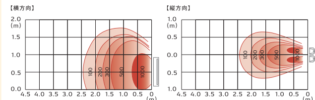
EU-30R
