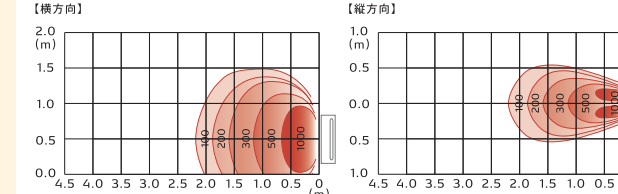
EG-15RK
