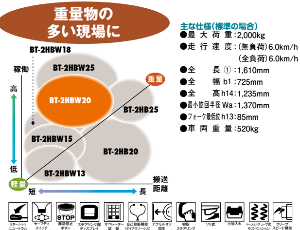
步行型2.0t BT-2HBW20
